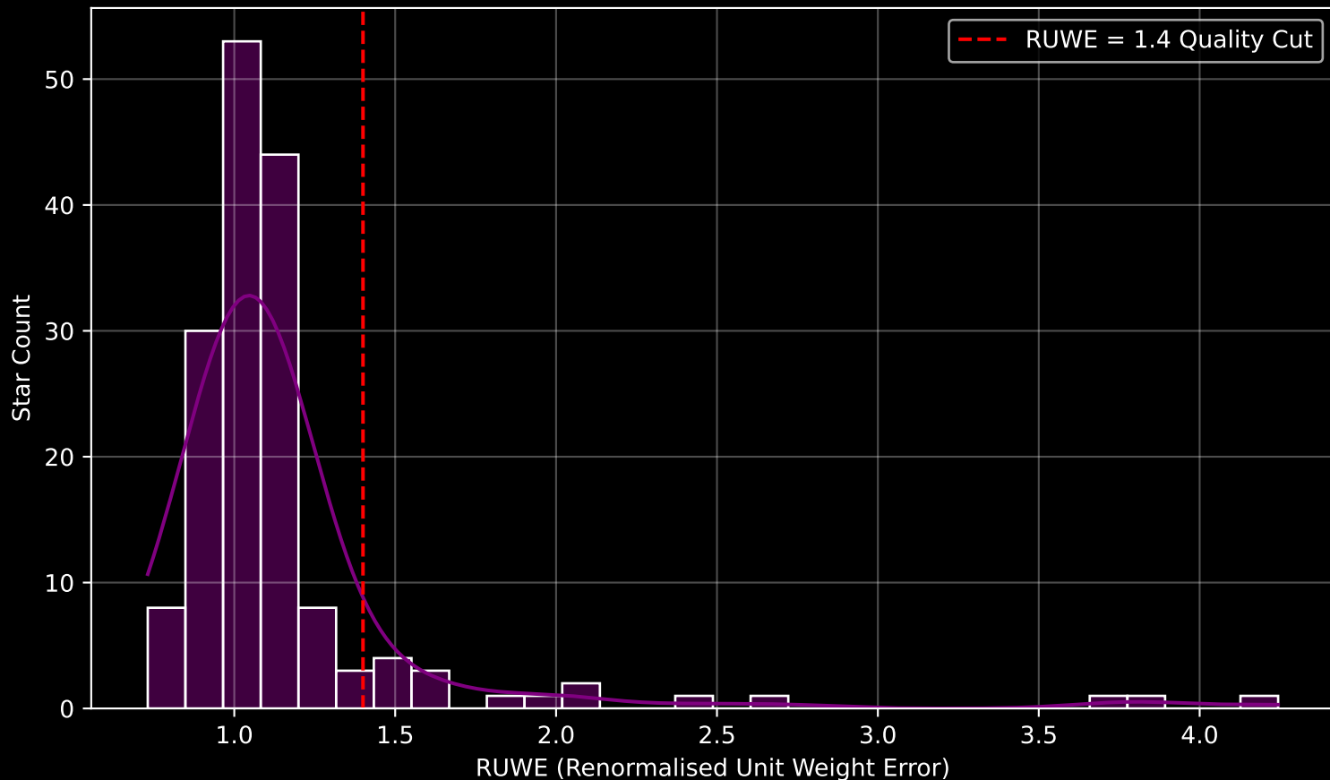
GAPOGEE DR17 Field [279-19-O_TESS] RUWE Distribution (n= 162)
