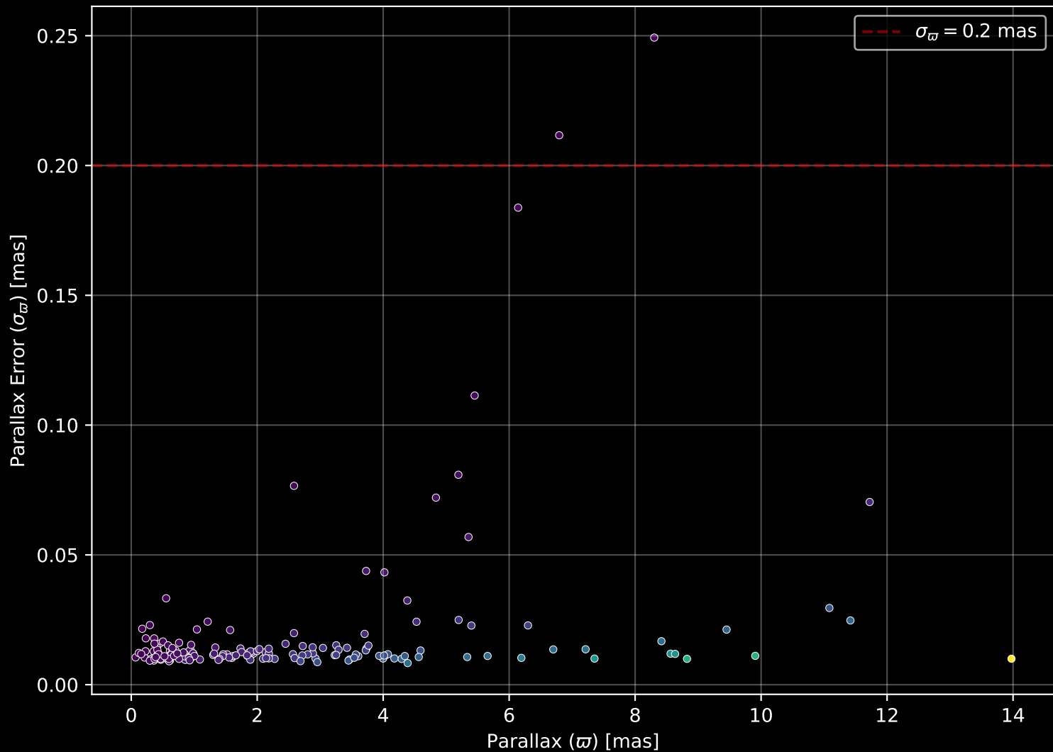
APOGEE DR17 Field: [279-19-O_TESS] Parallax Quality (n= 171)
