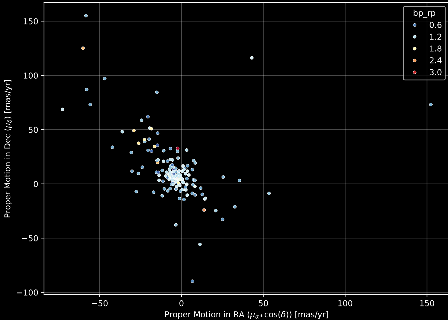
APOGEE DR17 Field: [279-19-O_TESS] Proper Motion Diagram (n= 171)
